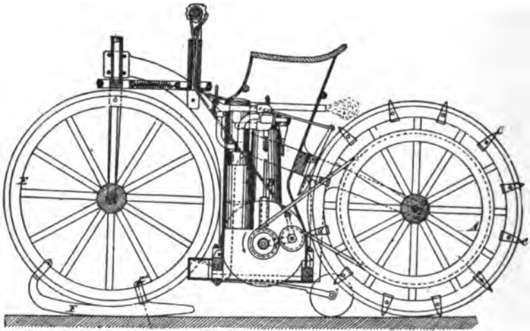
FIG. 388.—Sketch of Daimler's First Gasoline Propelled Bicycle. This machine is shown arranged for sliding on ice, having teeth, C, in the rear wheel, and the runner, F, secured to the forward wheel, E. A is the driving pulley on the rear wheel; B, the cylinder of the motor.
